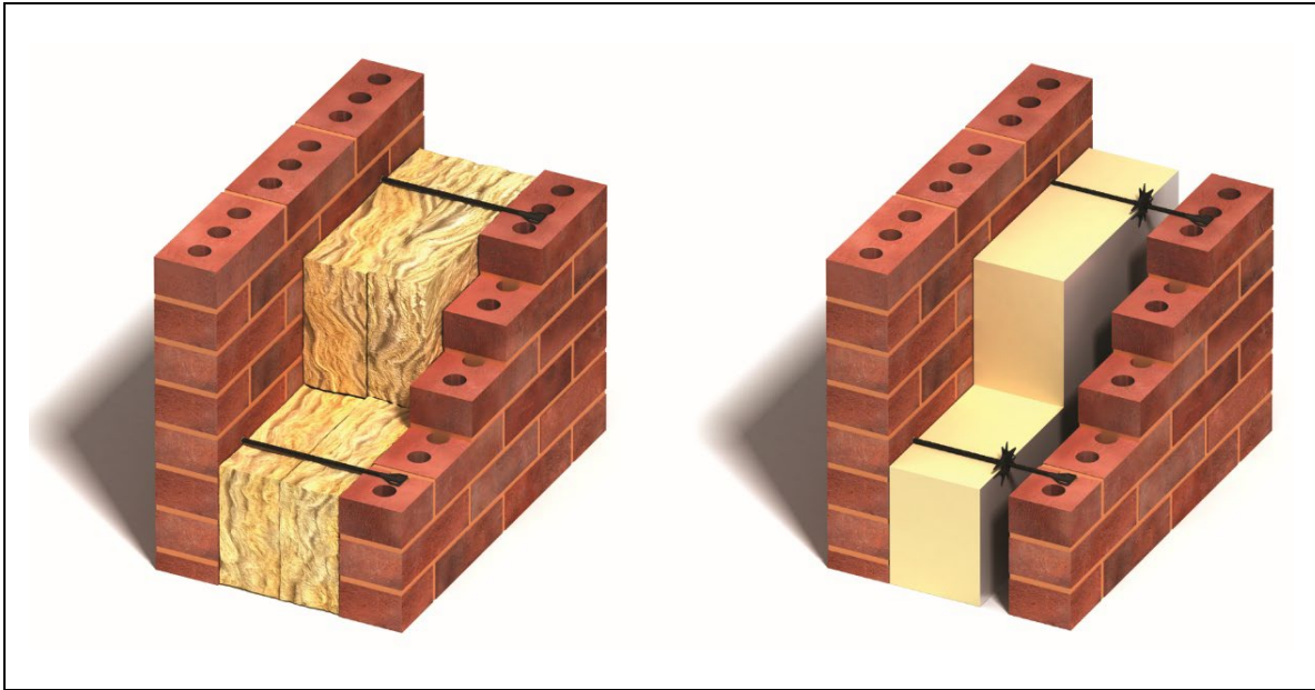
Figure 2b Typical installation details Teplo BF and BFR Wall Ties
