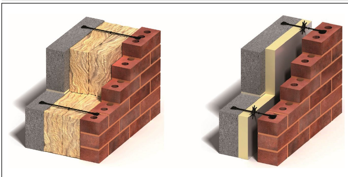
Figure 2a Typical installation details Teplo BF and BFR Wall Ties
