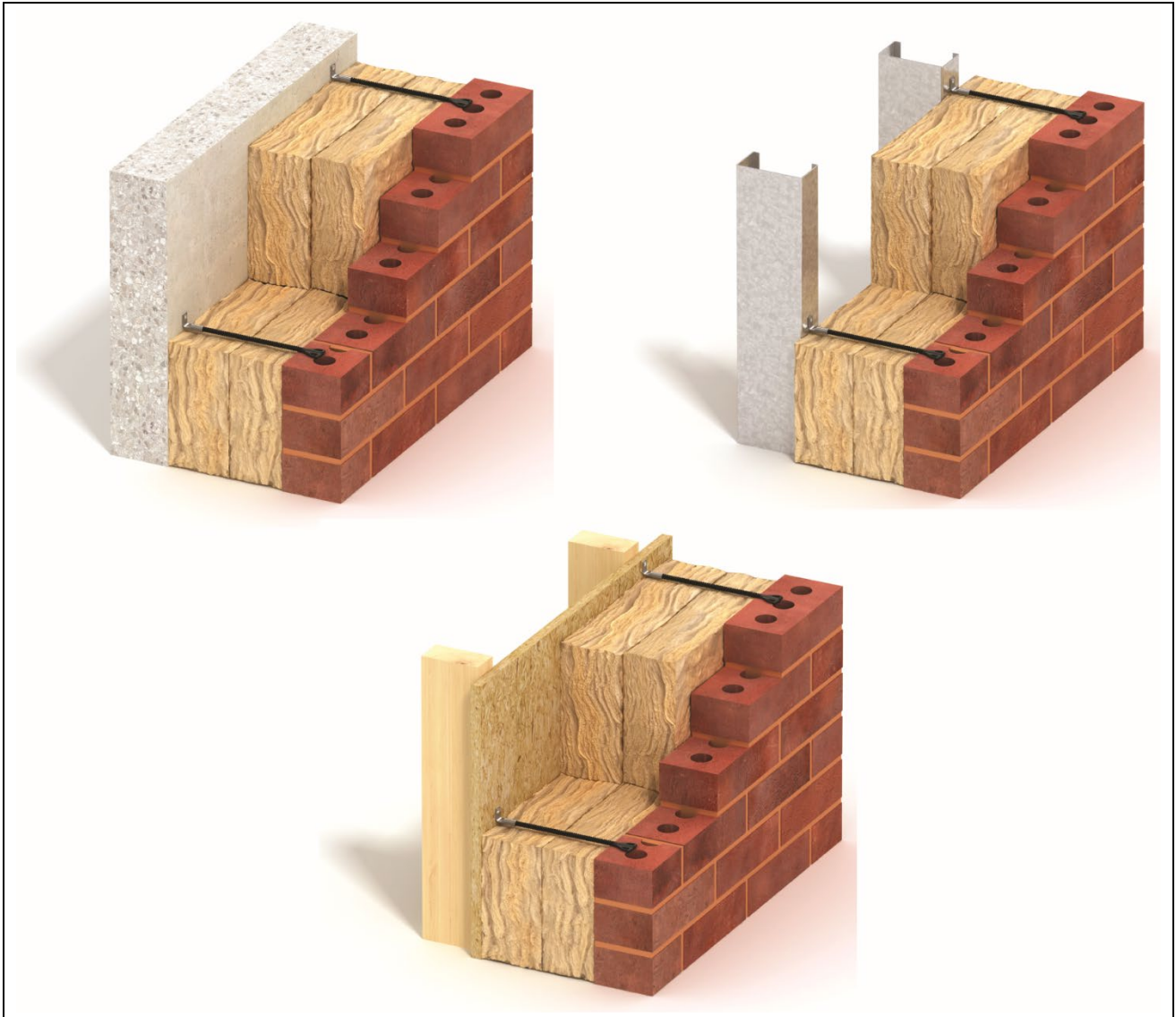
Figure 2 Typical examples of Teplo BFL Wall Ties in use
